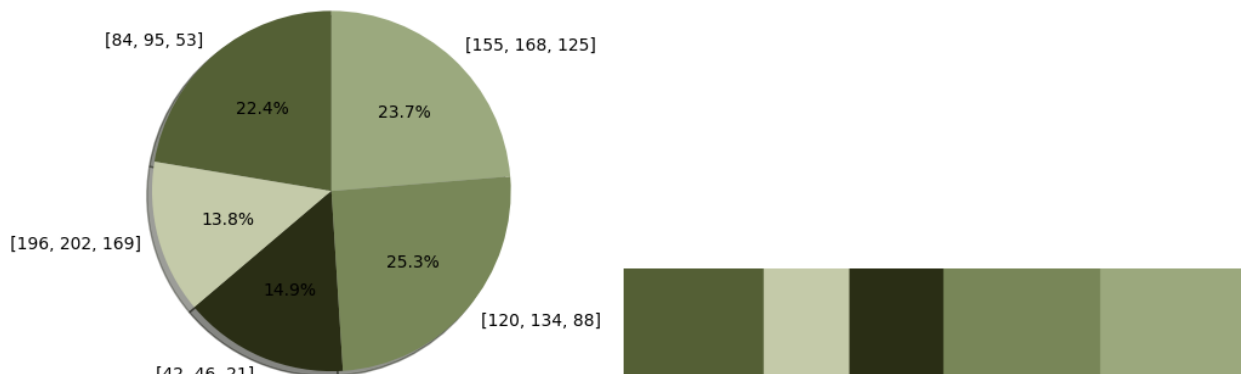
Figure 7: Illustration of spectrum of 5 dominant colors in term of the RGB values and frequency of occurrence in the input background image.
