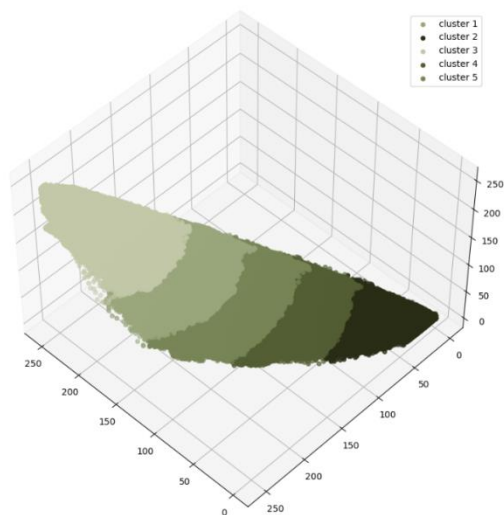
Figure 6: Clustering the vectorised feature into dominant colors using K-Means (K = 5).
