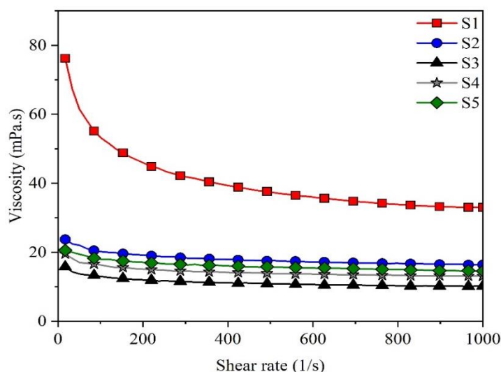
Figure 4: Viscosity as a function of shear rate of samples.
