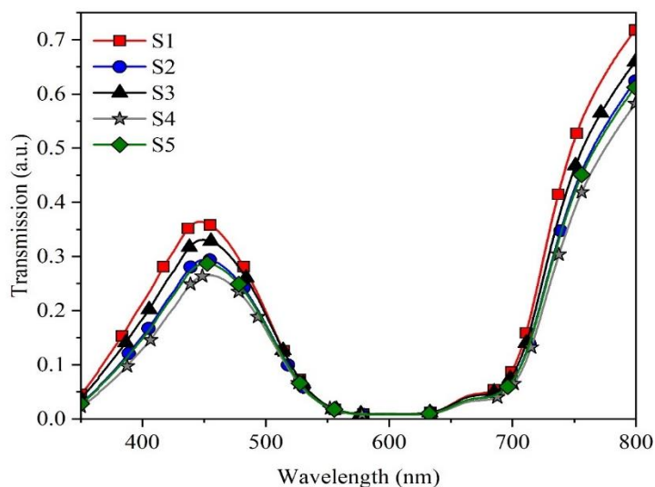
Figure 2: UV-Vis spectra of samples.
