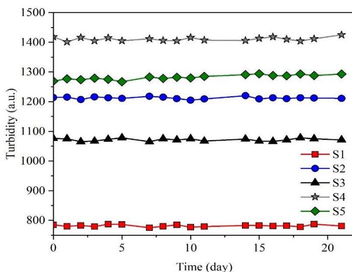
Figure 3: Turbidity of the samples during storage at ambient condition.
