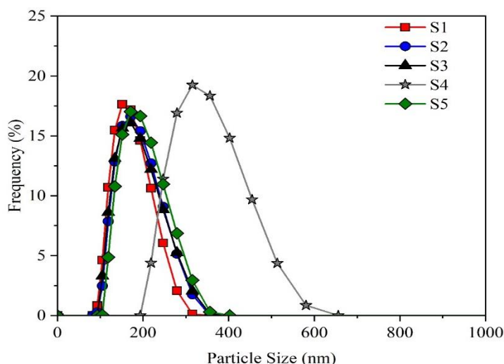
Figure 1: Particle size distribution of samples obtained by DLS.
