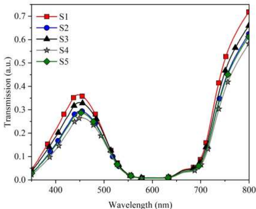
Figure 2: UV-vis spectra of samples.
