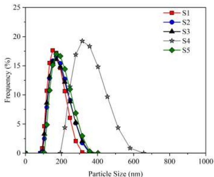
Figure 1: Particle size distribution of samples obtained by DLS.
