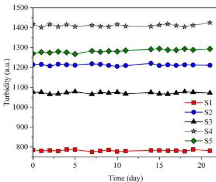
Figure 3: Turbidity of the samples during storage at ambient condition.
