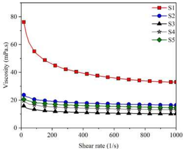
Figure 4: viscosity as a function of shear rate of samples.
