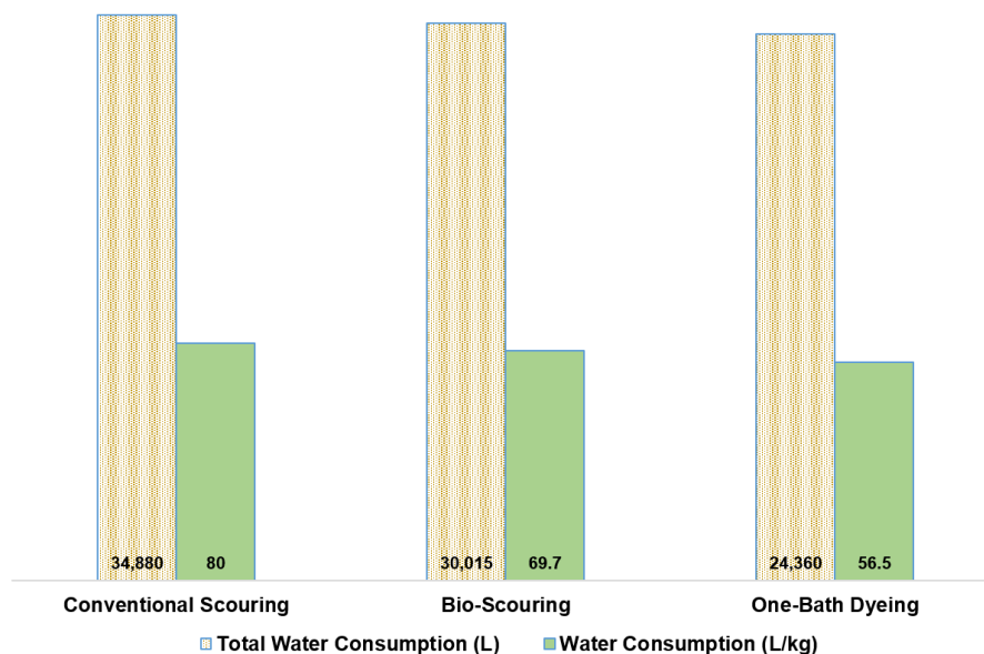
Figure 1. Total and specific water consumption of conventional scouring, bio-scouring, and one-bath dyeing processes.
