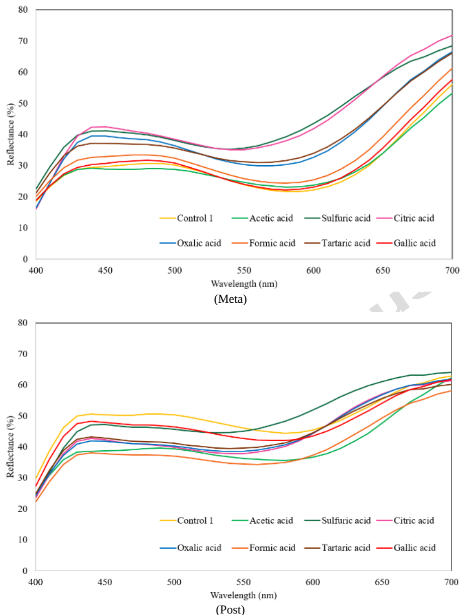
Figure 3. Reflectance spectra of fabrics dyed using different mordanting methods and acids
