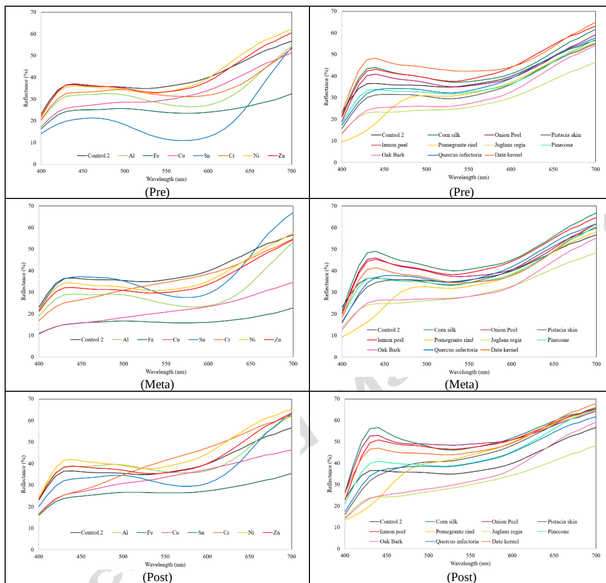
Figure 7. Reflectance spectra of fabrics dyed using different mordanting methods and mordants
