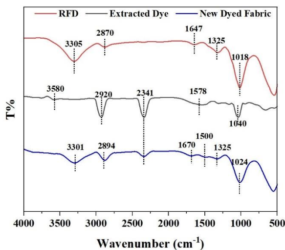
Figure 2: FTIR spectra of RFD (Ready for Dye), extracted dye, and dyed fabric.
