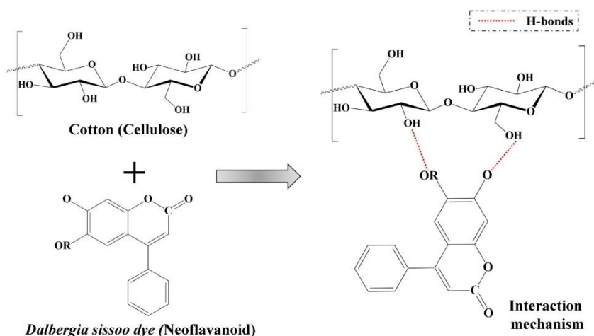
Figure 3: Possible bonding mechanics between the neoflavanoid of Dalbergia sissoo wood waste extract and cotton.
