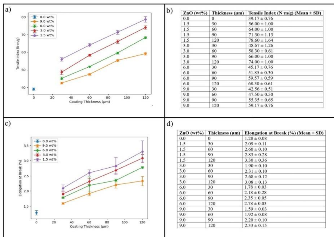
Figure 5: Effect of ZnO nanoparticles concentration and coating thickness on mechanical properties of papers coated with ZnO–CMC: (a) Evolution of tensile index with coating thickness at different ZnO concentrations, (b) Tabulated values of tensile index (mean ± SD), (c) Evolution of elongation at break (%) with coating thickness at different ZnO concentrations, (d) Tabulated values of elongation at break (mean ± SD).
