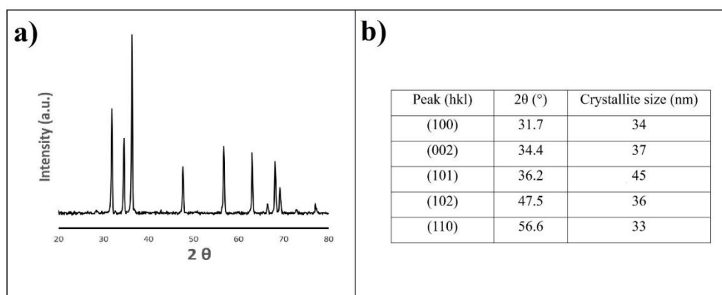
Figure 2: XRD results of synthesized ZnO; a) XRD patterns and b) Crystallite size of synthesized ZnO nanoparticles calculated using the Debye–Scherrer equation.
