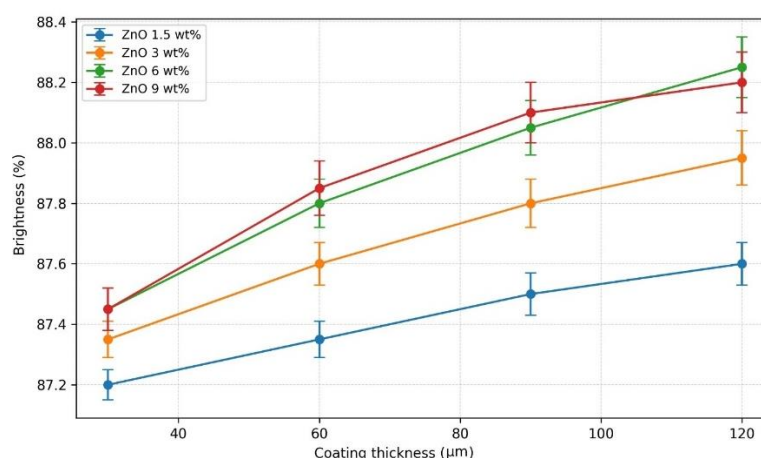
Figure 7: Brightness of papers with different coating thicknesses and different weight percentages of ZnO nanoparticles.
