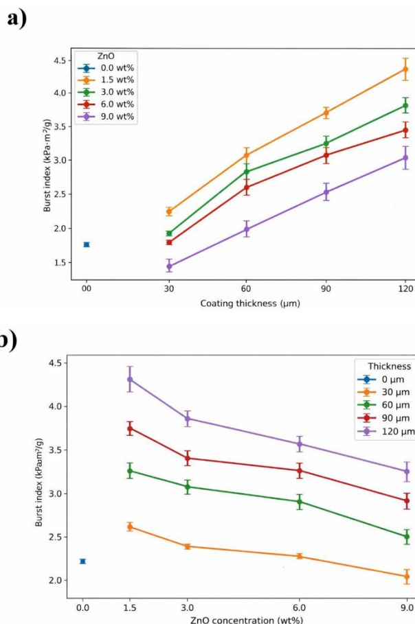
Figure 6: Effect of ZnO nanoparticles concentration and coating thickness on burst strength of papers coated with ZnO–CMC system: (a) Bursting index changes with coating thickness for different ZnO concentrations, (b) Bursting index changes with ZnO concentration for different coating thicknesses.
