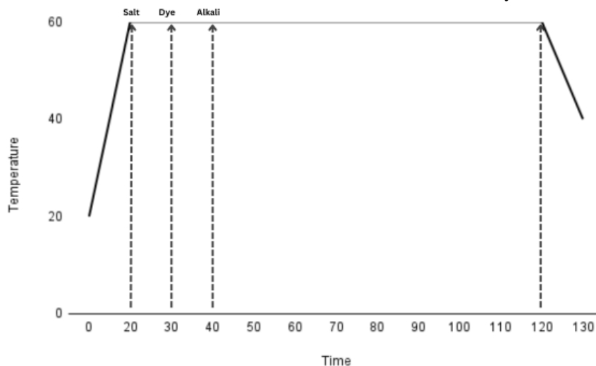
Figure 1: Reactive dyeing graph.
