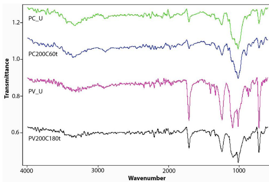
Figure 4: FTIR of treated PC and PV samples.
