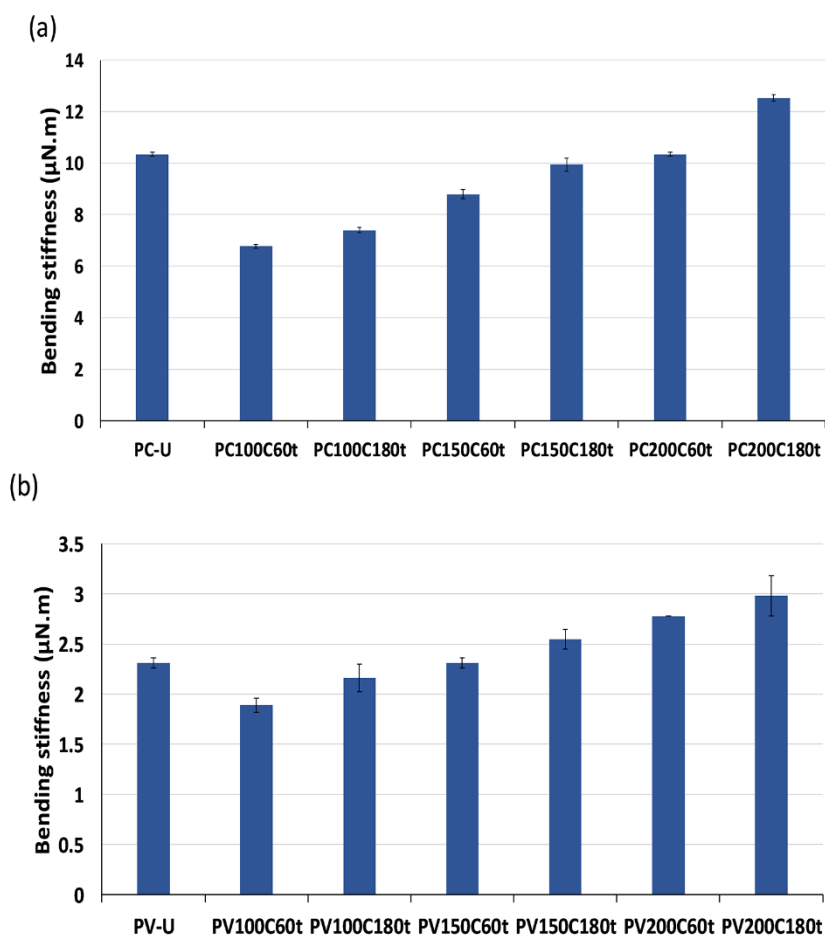
Figure 6: Bending stiffness of PC (a) and PV (b) samples.
