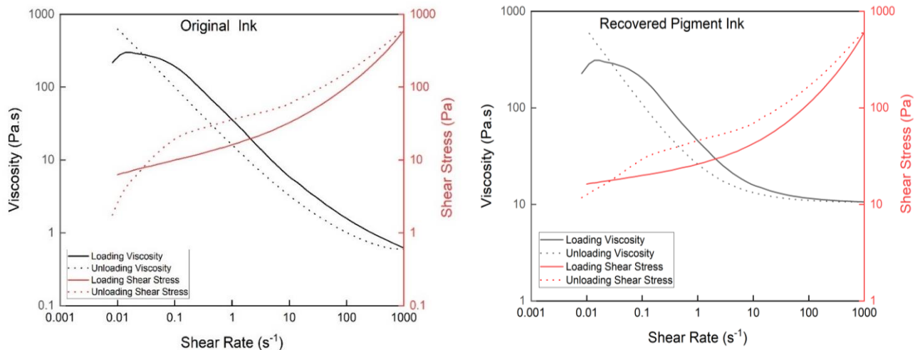
Figure 6: Viscosity and shear stress behavior of the original ink and the ink containing the recovered pigment.
