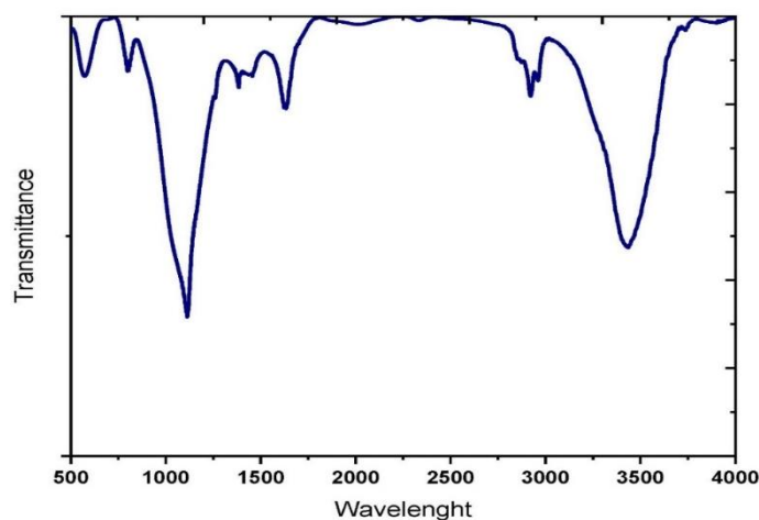
Figure 2: The FTIR diagram of the recovered pigment.
