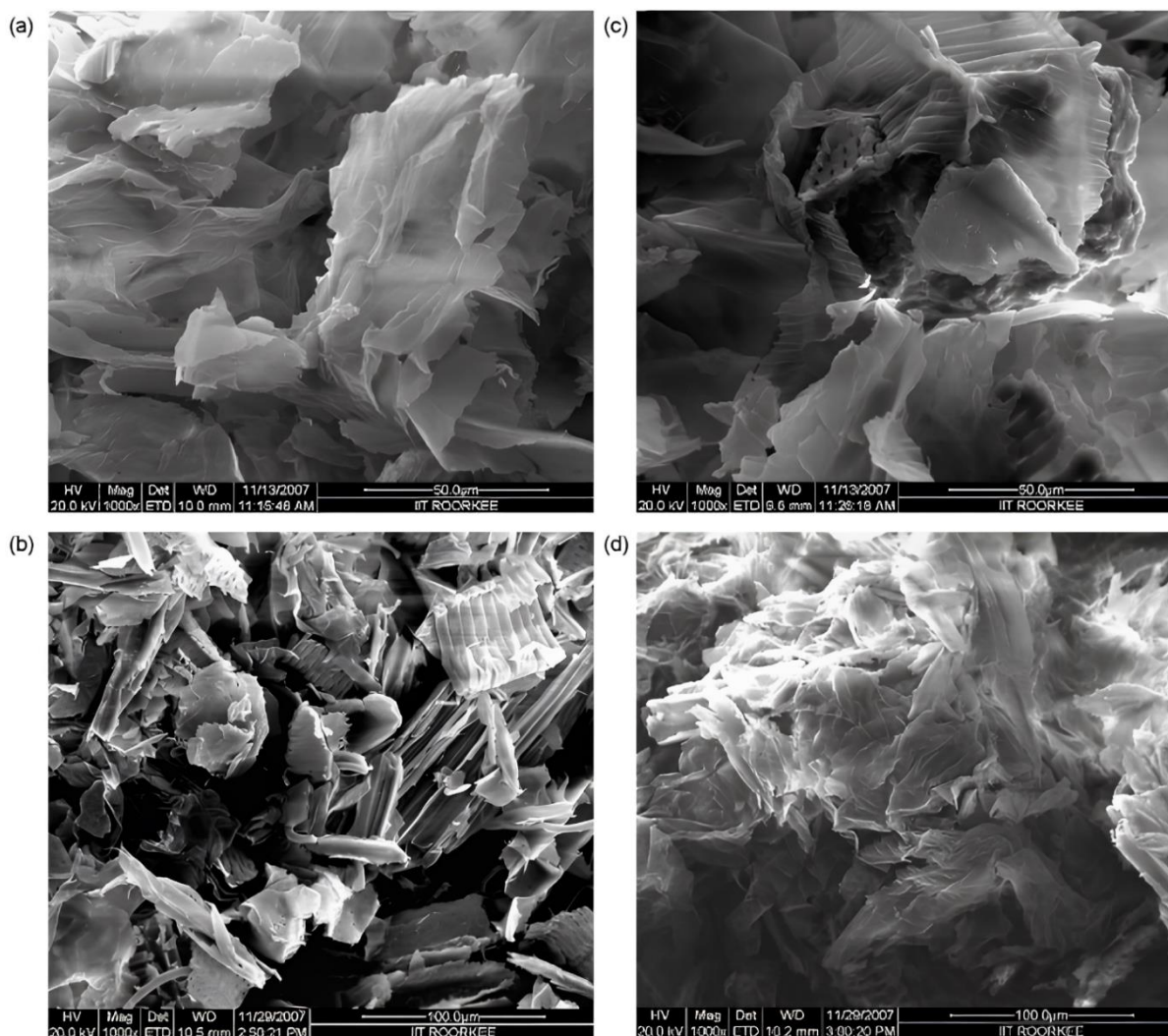
Figure 3: SEM images depicting various samples: (a) SEM images of untreated BSS, (b) SEM images of BSS loaded with Cr (VI), (c) SEM images of untreated FSS, and (d) SEM images of FSS loaded with Cr(VI) [53]. (Reprinted with permission from [53]. Copyright 2009; Elsevier publishing due to open access).
