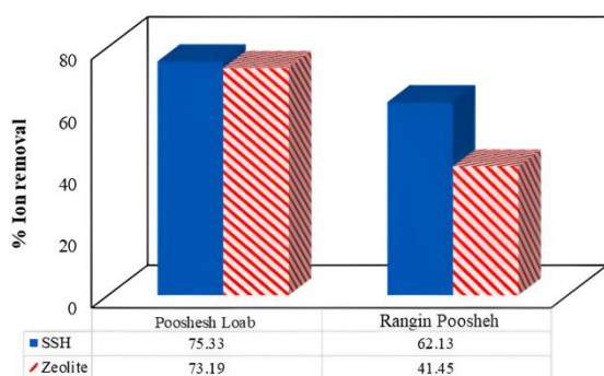
Figure 4: A comparison of the percentage of Ni(II) ion removal from industrial wastewater samples using SSH and Zeolite [54]. (Reprinted with permission from [54]. Copyright 2023; Elsevier publishing due to open access).
