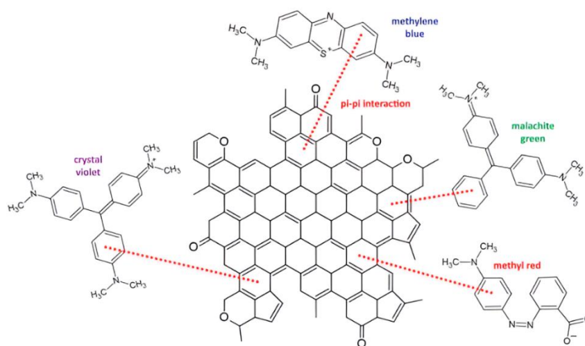
Figure 6: Organic dyes adsorption on activated carbons [59]. (Reprinted with permission from [59]. Copyright 2022; MDPI publishing due to open access).
